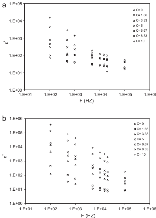
Fig. 9. Variation of (a) dielectric constant \epsilon' , (b) dielectric loss \epsilon'' with frequency for PVA: C (NaI/CuCl 2 ) polymer electrolytes at 303 K.
