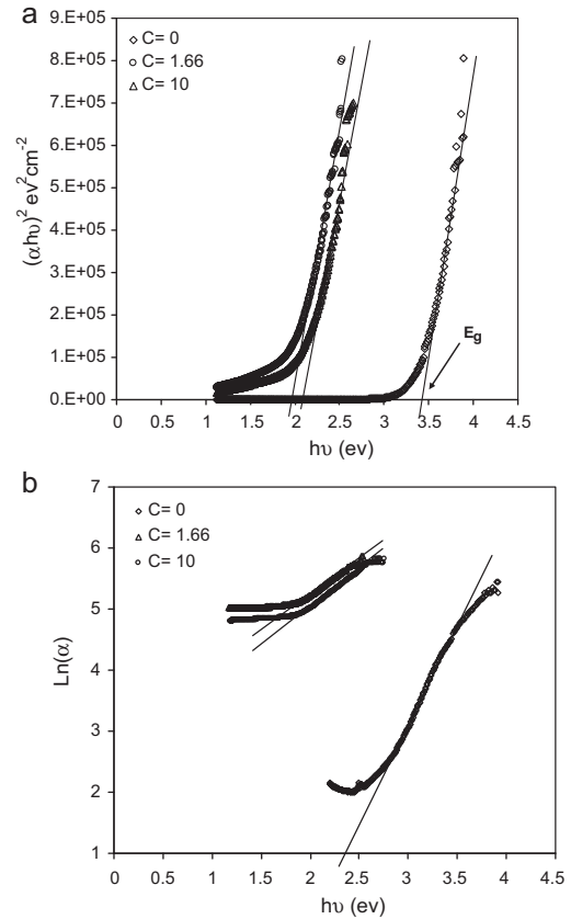
Fig. 11. The dependence of (a) (\alpha h\nu)^2 , (b) \ln(\alpha) on the photon energy h\nu .
